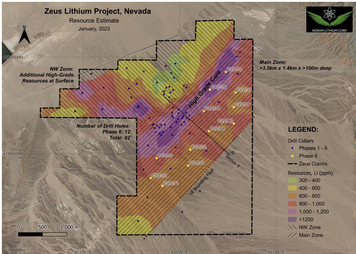
Plan view of lithium grade distribution
